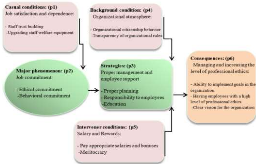
Fig. 1: Research model
